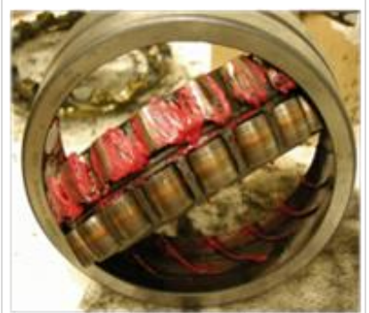
Spherical Roller Bearing
