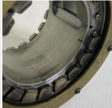
Journal/Thrust Bearings
